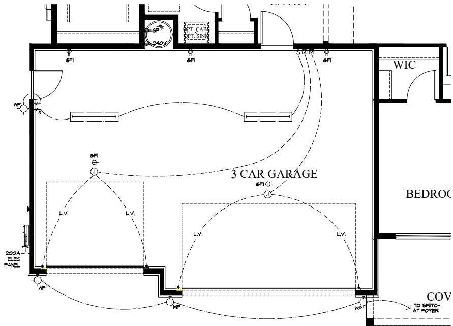
Partial Elec Plan - Opt. Front Load Garage
