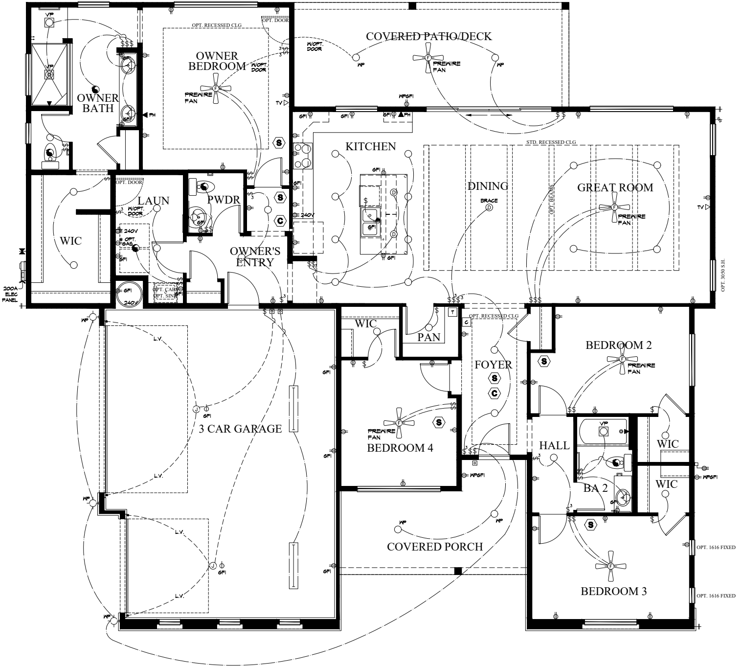
Elec Plan (All Elevs Similar)
