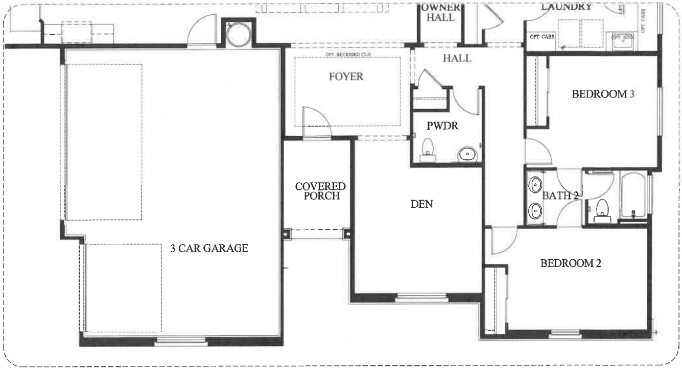
Partial Plan - Elev B
