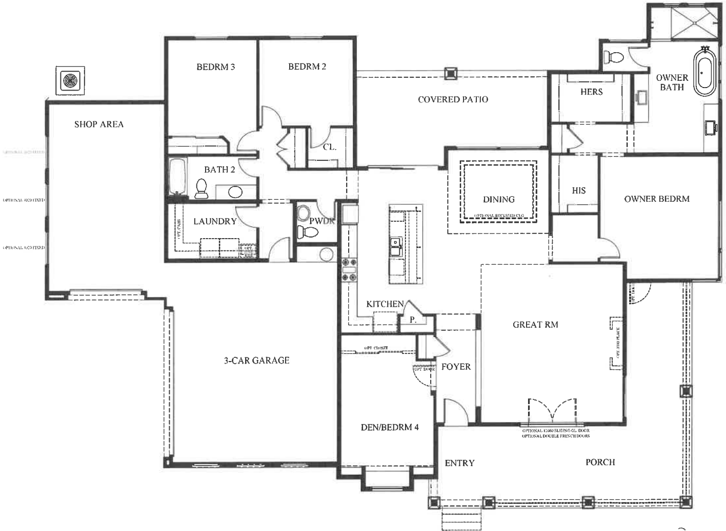
Plan - Elev A
